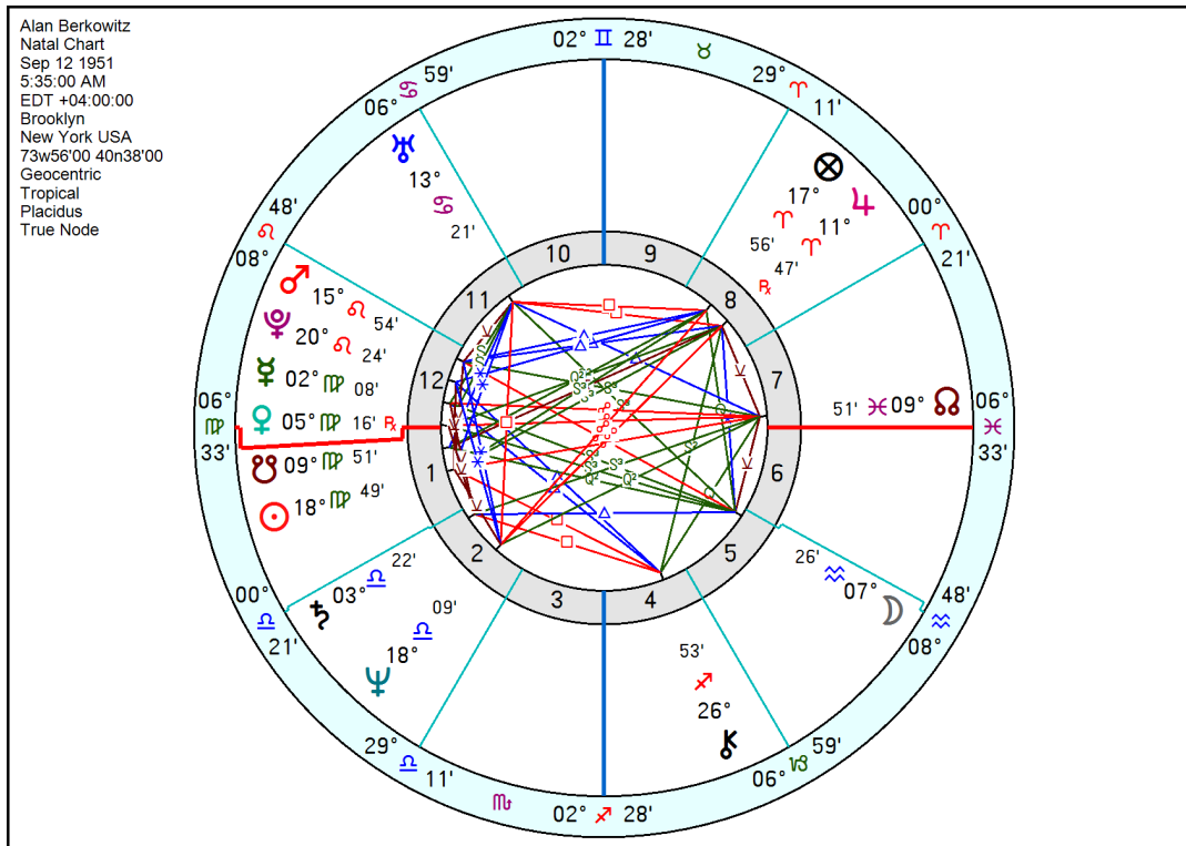
FIGURE 1982 0322c-1. Alan Berkowitz Natal Chart (computer generated, Janus 5). POF [Part of Fortune] night formula used. [Note: The POF night formula was not used in WG classes, thus resulting in a different POF for individuals with Sun below the horizon.]
