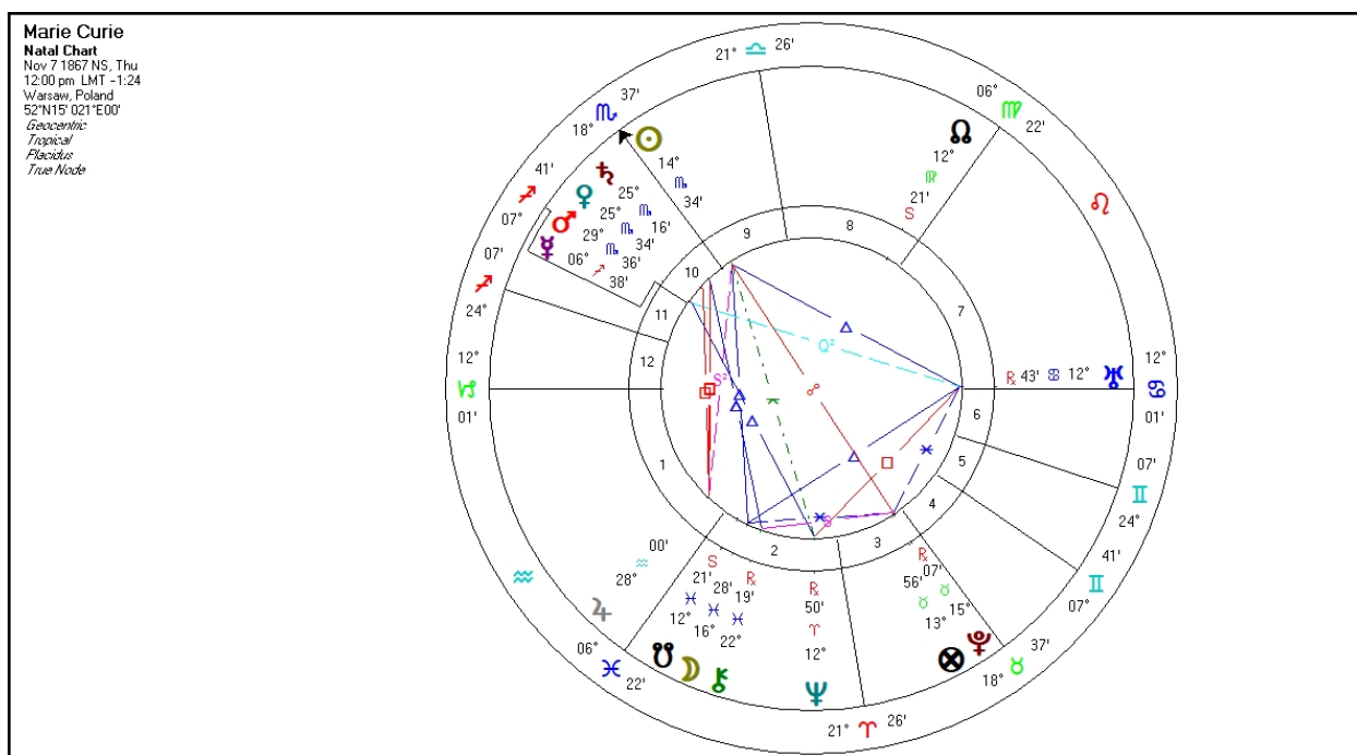
FIGURE 1983 0430b-1. Marie Curie Natal Chart (computer generated, Solar Fire); birth data from astro.com.
