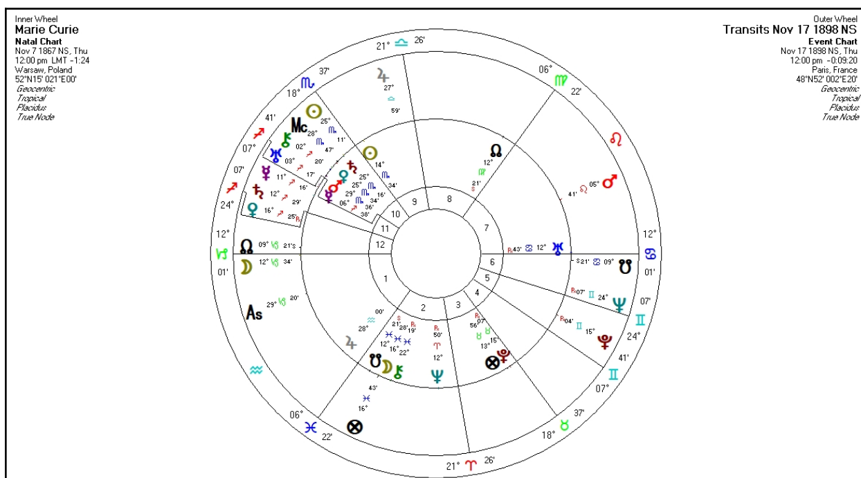
FIGURE 1983 0430b-2. Suggested Transits for Isolation of Radium Line in Spectrograph (computer generated, Solar Fire)
